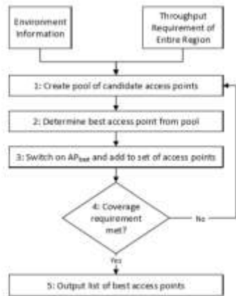
Fig. 2 shows the algorithm flow.
